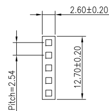
HOUSING
