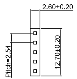
HOUSING
